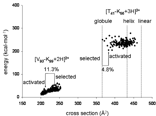
Figure 6. Plots of energy versus conformer cross section of the 150 lowest-energy structures post simulated-annealing for two peptides from Figure 5: [V_{93}-K_{99}+2H]^{2+} and [T_{41}-K_{56}+3H]^{3+} , as well as cross sections of the energy-minimized structures of the [T_{41}-K_{56}+3H]^{3+} ion modeled as a helix and linear structure, denoting the range of structures available to each sequence. Cross sections of the selected and activated structures for each sequence are highlighted, along with percent shifts from the mobility-selected structure. Peptide nomenclature is the same as in Figure 5.
