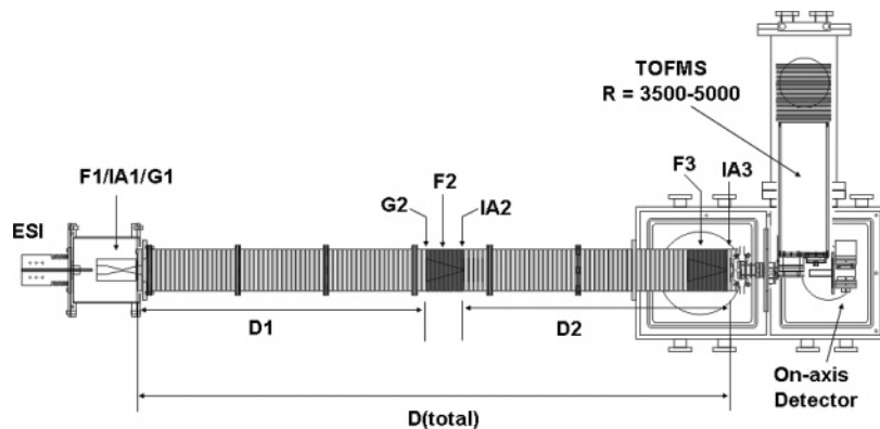
Figure 1. Schematic of the IMS–IMS–TOF instrument. Ions are gated through G1, where they undergo mobility separation in D1. Ions can be selected on the basis of mobility at G2. Ion activation is carried out at the region labeled IA2. For more detail on ion selection and activation, refer to text.
