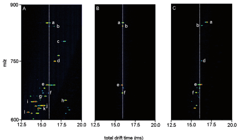
Figure 4. Nested drift (flight) time distributions for horse myoglobin tryptic digest, total distribution (A, left), ions mobility selected at G2 ( t_{D1} = 7.55\text{--}7.65 ms) with IA2 = 0 V (B, center), and same selection with IA2 = 120 V (C, right). The dotted lines denote the arrival times for inactivated mobility-selected ions, to show the degree of separation. a, [G_1\text{--}R_{31}+4H]^{4+} ; b, [Y_{103}\text{--}K_{133}+4H]^{4+} ; c, [K_{63}\text{--}K_{78}+2H]^{2+} or [H_{64}\text{--}K_{79}+2H]^{2+} ; d, [H_{119}\text{--}K_{133}+2H]^{2+} ; e, [H_{64}\text{--}K_{67}+2H]^{2+} ; f, [V_{68}\text{--}K_{77}+2H]^{2+} ; g, [K_{79}\text{--}K_{96}+3H]^{3+} ; h, [L_{32}\text{--}K_{47}+3H]^{3+} ; i, [L_{32}\text{--}K_{42}+2H]^{2+} ; j, [Y_{103}\text{--}K_{118}+3H]^{3+} ; k, [G_{80}\text{--}K_{96}+3H]^{3+} ; l, [E_{148}\text{--}G_{153}+H]^{+} . Note that the nomenclature used refers to the position of the peptide by providing the location (with respect to the intact protein sequence) and single letter abbreviation of the N- and C-terminal residues, respectively.
