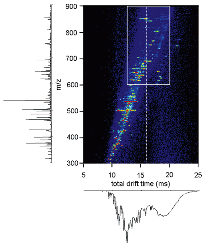
Figure 3. Nested drift (flight) distribution for electrosprayed horse myoglobin tryptic peptides, obtained by allowing all ions to traverse the whole drift tube, along with the integrated mass spectrum and drift distribution. The white box highlights the range examined in Figure 4.
