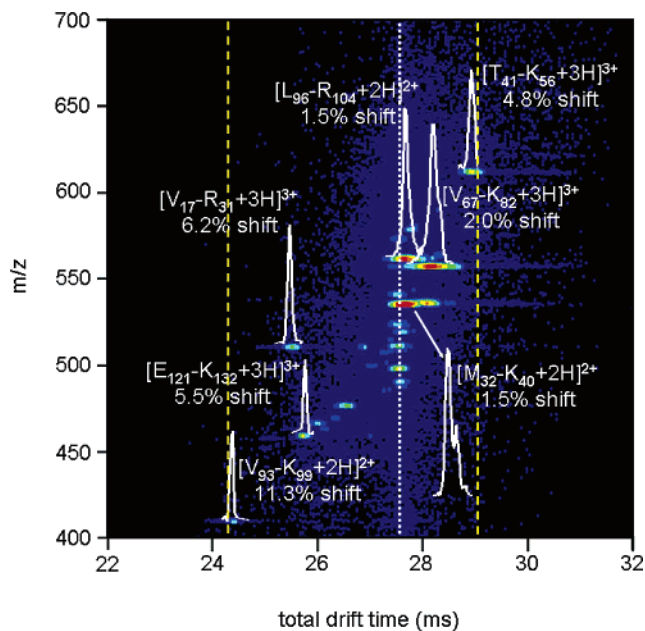
Figure 5. Expanded view of an activated selection of human hemoglobin tryptic peptides with t_{D1} = 9.366 ms. The white dashed line denotes the time at which mobility-selected ions with no activation are observed, while the dotted yellow lines show the new effective separation space of the second IMS experiment ( \sim 4.8 ms). Drift slices for several peptides are shown, along with shifts from original (inactivated) drift times for all ions. Peptide nomenclature is carried out the same as in Table 1 and Figure 4.
